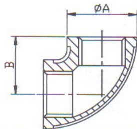
Elbow 90°
