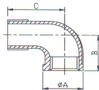
Street Elbow
