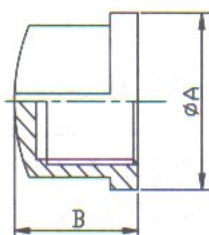
Round Cap
