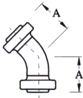
45° Bend MxM
